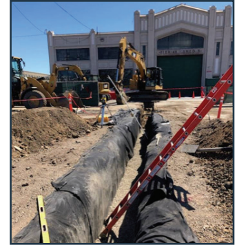
Trenching for temporary storm drains
